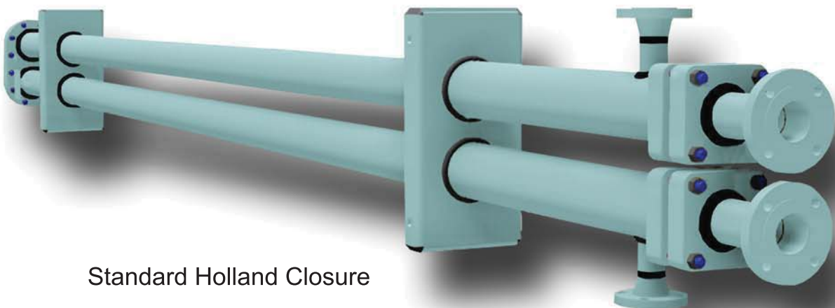
Separated Head Closure
