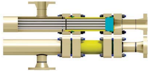
Holland separated head closure. Separate flanges and bolting for each gasket surface.
